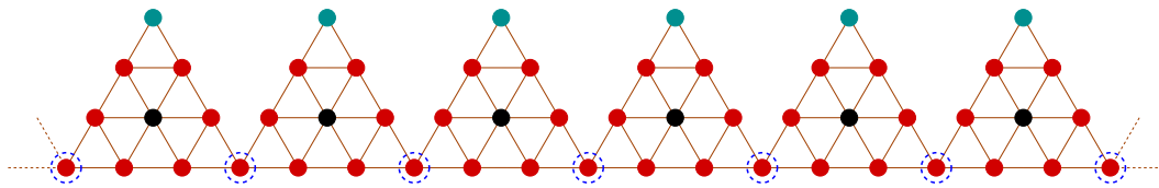
FIG. 5: (Color online) A periodic array of finite generation b = 3 SPG networks. With increasing generation each unit cell will be representative of an infinite SPG network.
